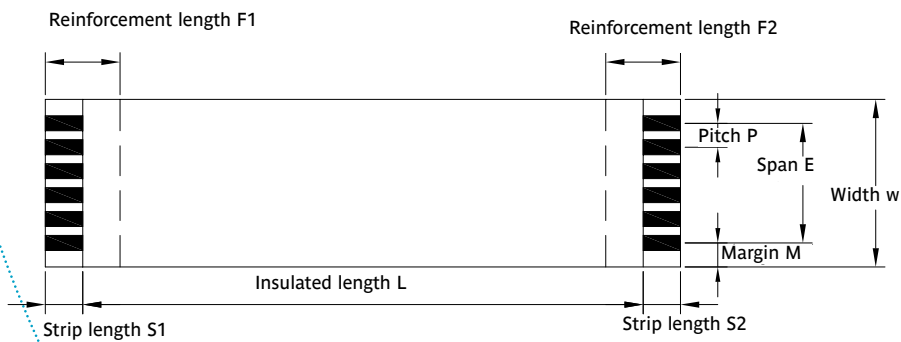
▲ CRIMPED CONTACTS
