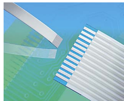
▲ 0.3 mm PITCH VERSUS 2.54 mm PITCH
