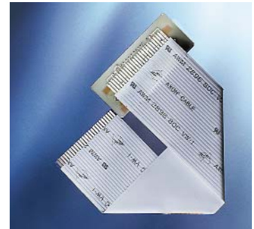
▲ FOLDED AND SOLDERED
