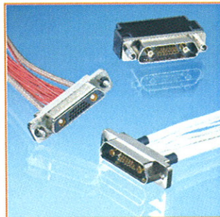
Combo connectors, connectors including signals, coaxial and power contacts
